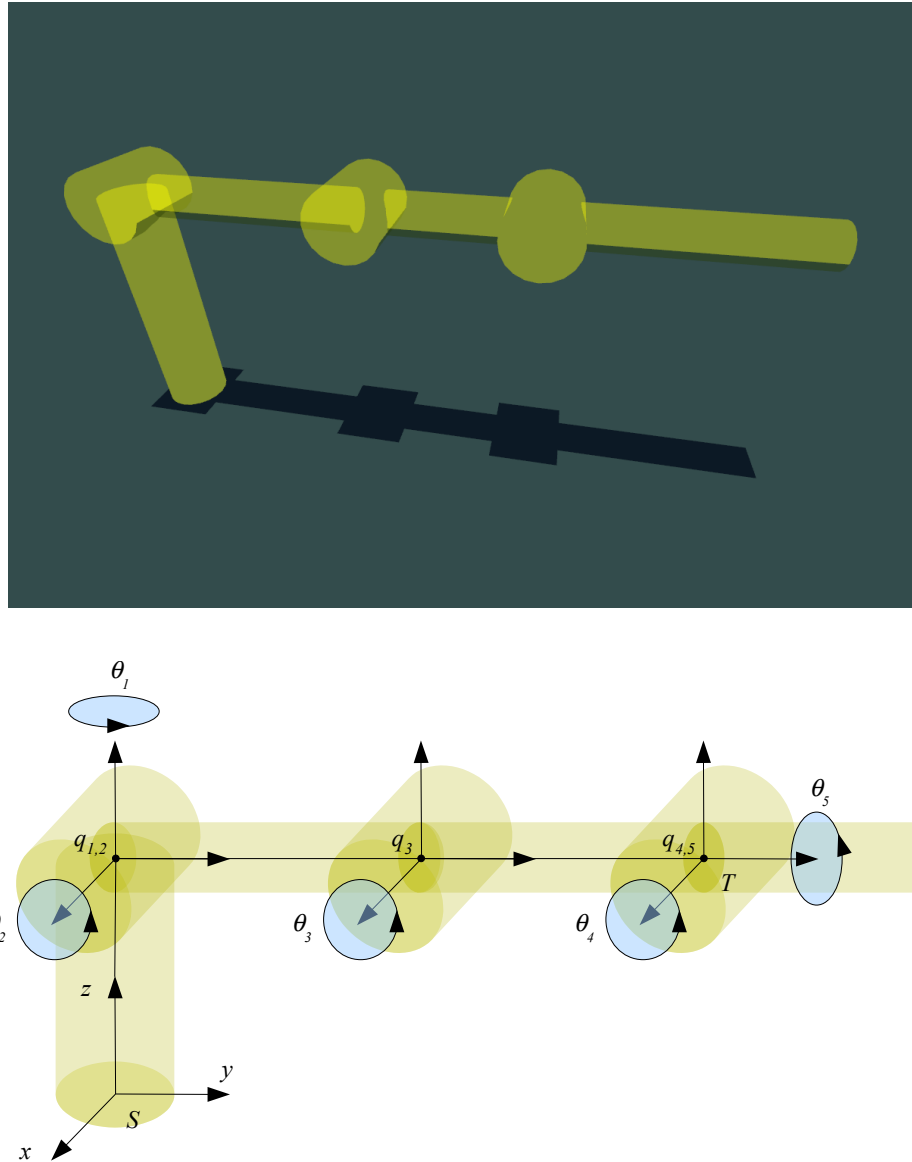
Figure 4.3: The Katana 6M180 manipulator (without a gripper) at the reference configuration in the Golem virtual environment in the top panel. The Katana model in the bottom panel shows base frame S , tool frame T , and the 5 axes of rotation of revolute joints with corresponding joint variables \theta_i and points q_i (see definition of twist in Appendix A.3.2).
