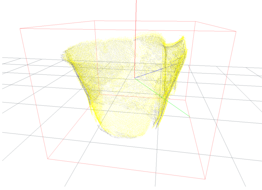
Fig. 3. The image shows the target object to be grasped. In this case the object is a jug. The grey point cloud represents the ground truth pose of the object, as it was acquired by a noiseless input source. The yellow point cloud identifies the best pose estimate. The yellow point cloud is organised as a KD-Tree for faster collision detections. The red box represents the bounding box which avoids unnecessary collision checking between the object and robot's links when they are far apart.
