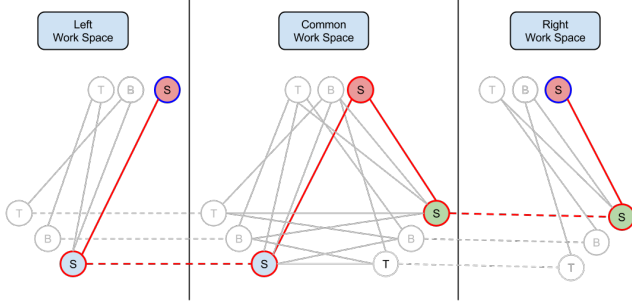
Fig. 8: Planning given by Dijkstra algorithm, the transition on the table is used because it is the shortest one in this example of initial and final states.
