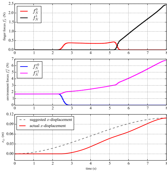
Fig. 4. Trajectories for a circular object manipulated by two independent fingers: normal contact forces f_N^i applied by the fingers; normal contact forces f_N^e applied by the environment (segments e_0 , e_1 ); suggested and actual x -displacement x of the object.
