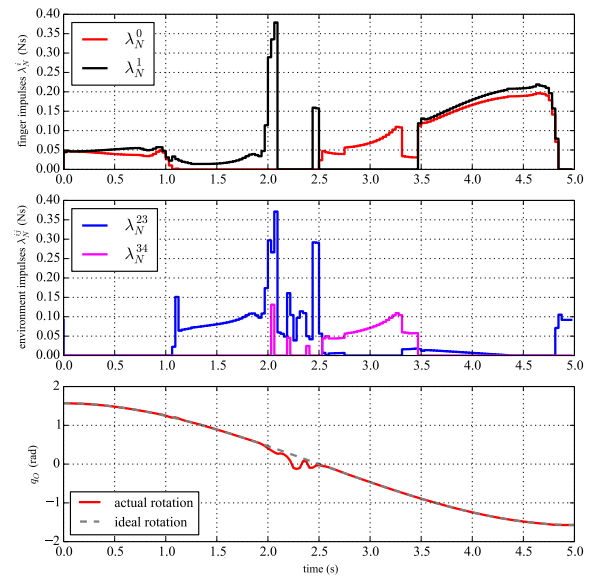
Fig. 6. Motion trajectories of a capsule-shaped object manipulated by an underactuated gripper: contact normal impulses \lambda_N^i applied by the fingers; contact normal impulses \lambda_N^e applied by the environment through segment P_iP_j ; ideal and actual rotation q_O of the object-fixed frame.
