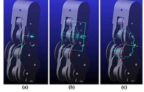
Fig. 5. Implementation of the SR joint in ADAMS: a virtual link is introduced between the two elements (a); a revolute joint connects the virtual link with each real parts (b); a gear-wheel constraint is imposed between the two revolute joints (c).
